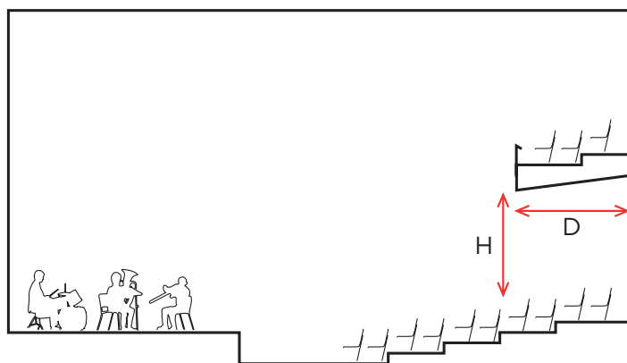
Figure 5.14: Recommended balcony overhang proportions: the depth D should not exceed the height H
