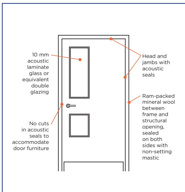
Figure 5.7: Desirable features of an acoustic door installation
