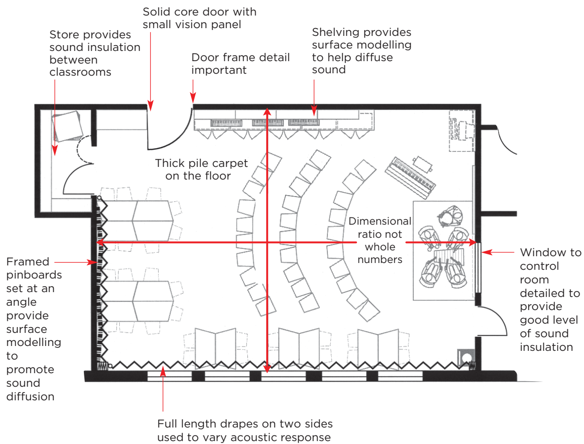
Figure 5.9: Acoustic treatment to music classroom/recital room
