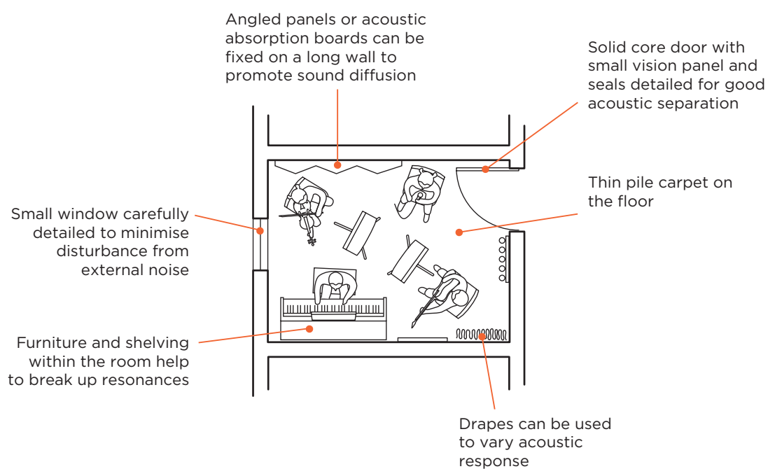
Figure 5.10: Acoustic treatment to 8 m² group room with parallel walls
