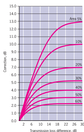
Figure 3.5 Chart to estimate R_w for a composite wall consisting of two elements with different transmission losses
