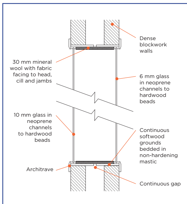
Figure 5.6: Section through control room window
