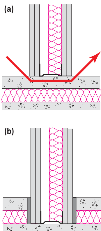
Figure 3.3 Flanking transmission via floating screed (a) Sound insulation may be limited by continuous screed (b) Higher sound insulation performance possible
