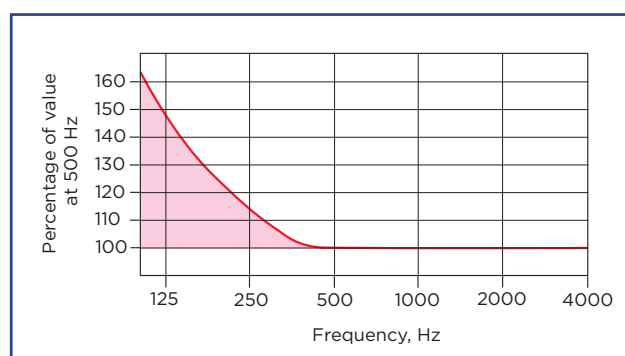
Figure 5.3: Recommended percentage increase in reverberation times at lower frequencies for rooms specifically for music
