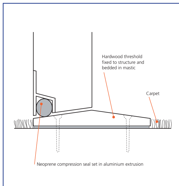
Figure 5.8: Example of acoustic door threshold seal
